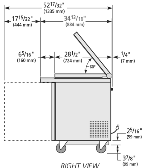
RIGHT VIEW
