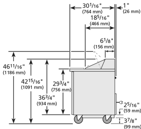
RIGHT VIEW
