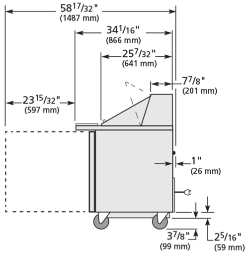
RIGHT VIEW
