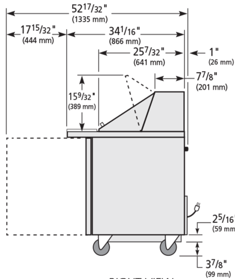
RIGHT VIEW
